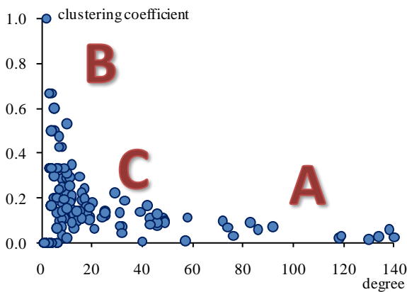
Figure 4 Clustering Coefficient and Degree
